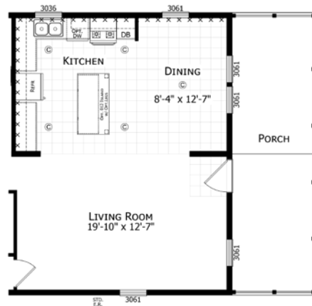
Opt. Porch
