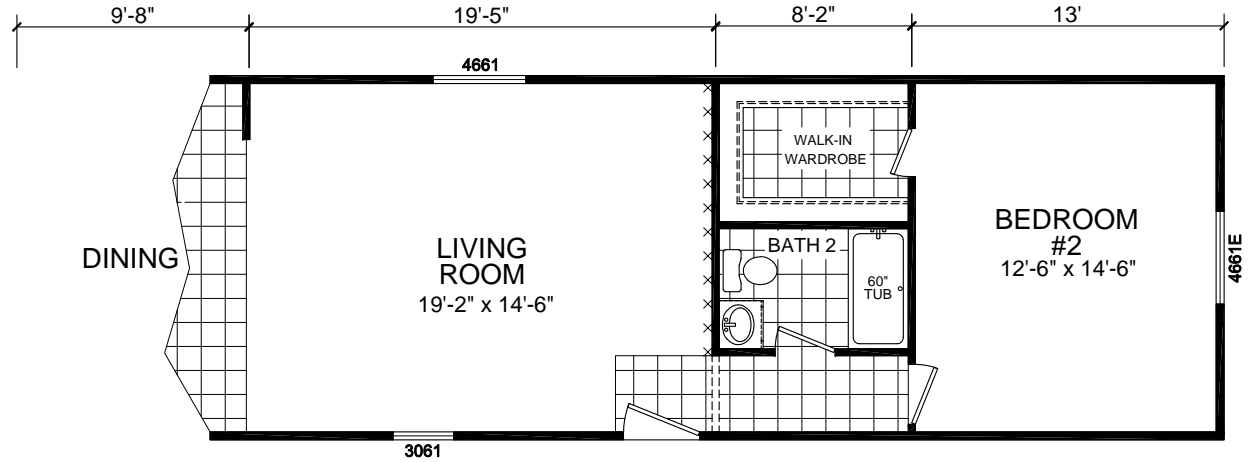
2 BEDROOM OPTION
