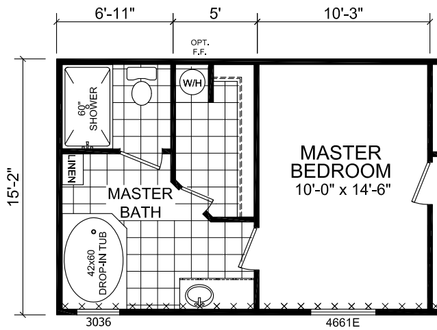
OPT. MASTER BATH
